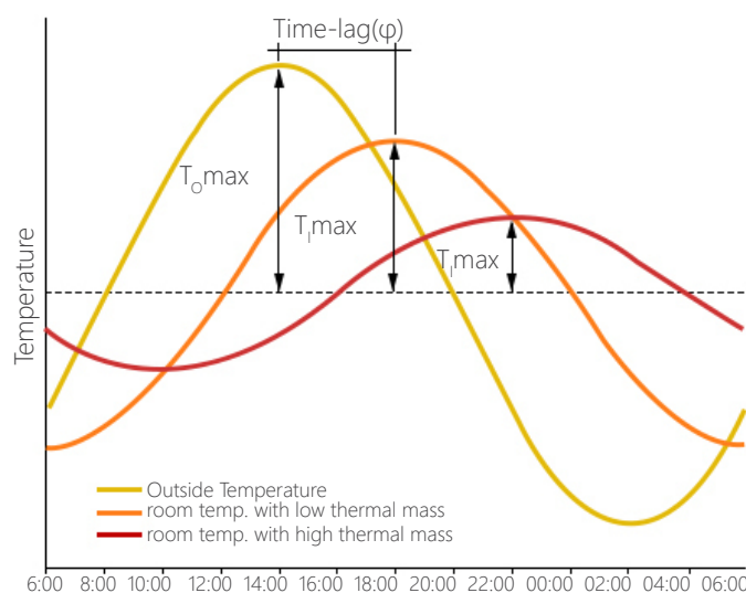
Figure 35: Thermal mass of a building affects increases the time taken by heat to flow from outside to inside
