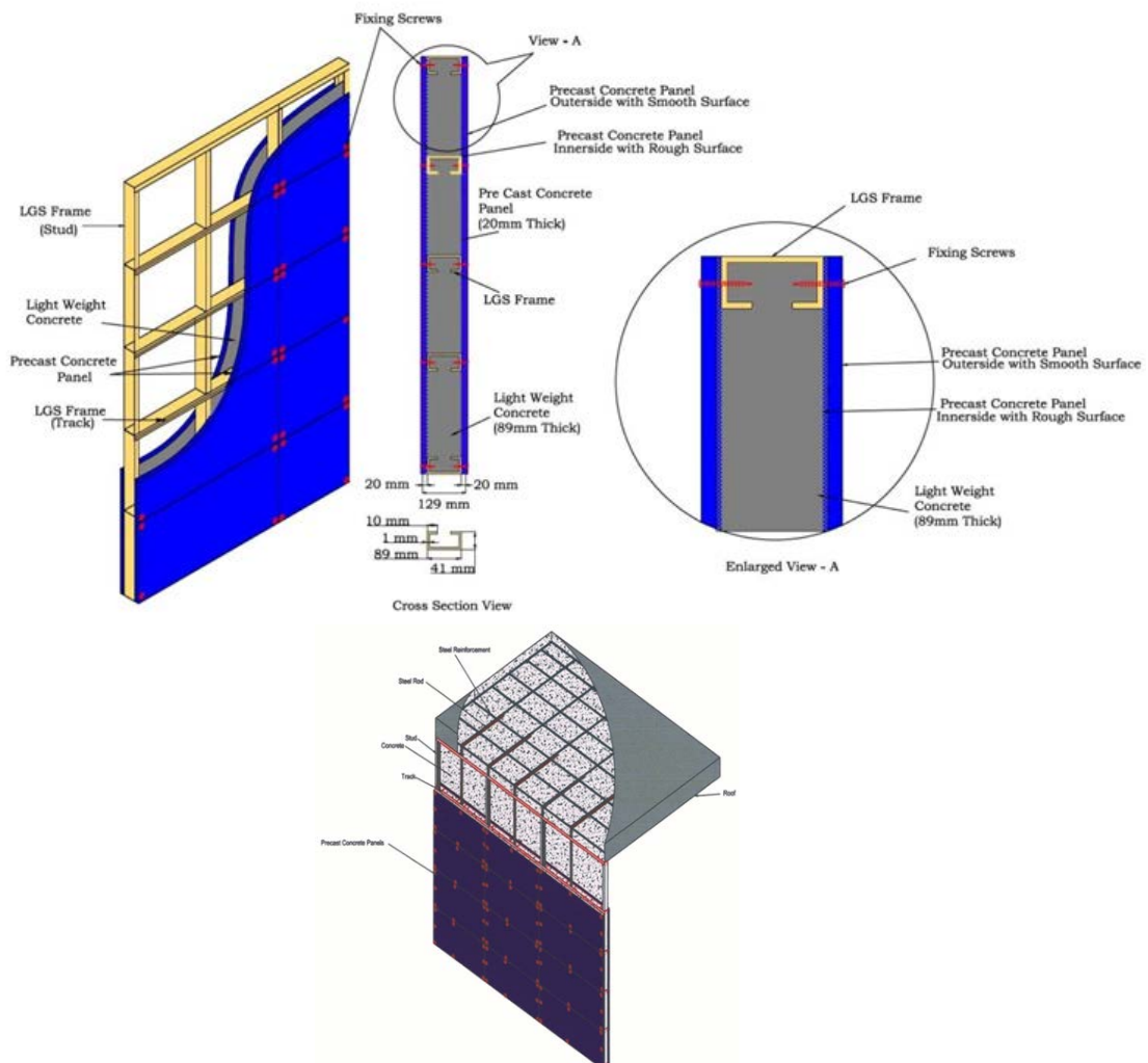
Figure 102: Structural Details of LGSFS-Infill Concrete Wall. Source: (MoHUA, GoI, 2021)
