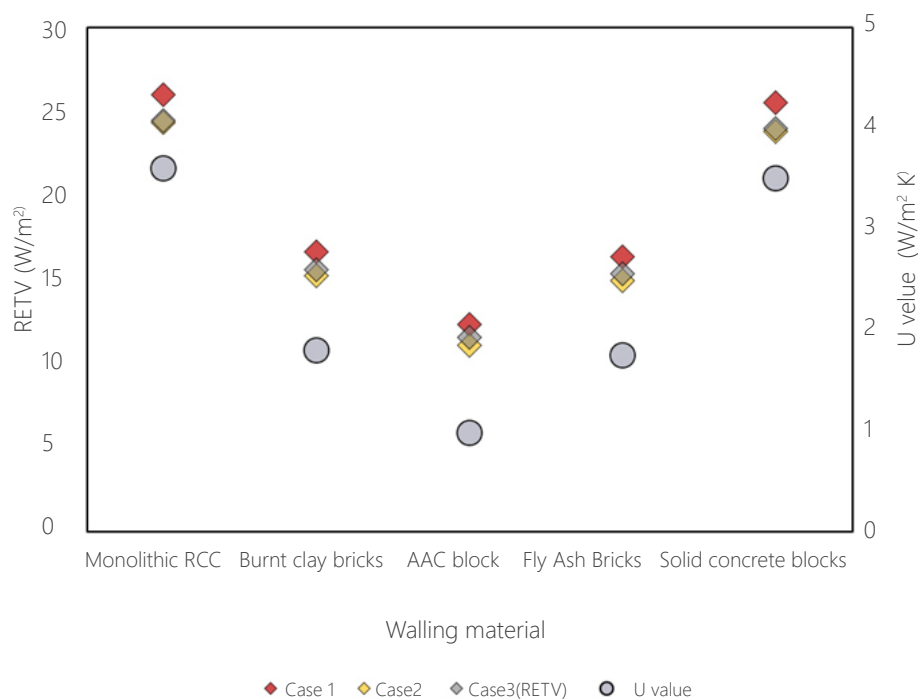
Figure 144: U-value and RETV for walling materials
