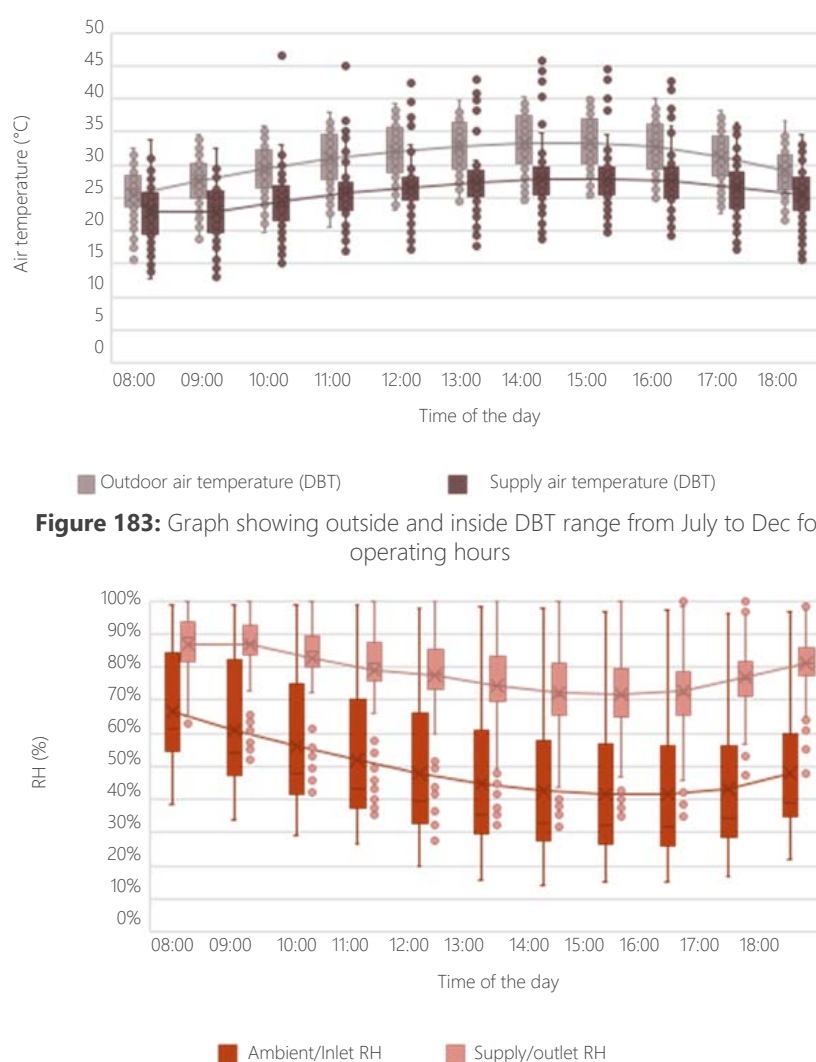
Figure 184: Graph showing outside and inside RH range from July to Dec for operating hours
