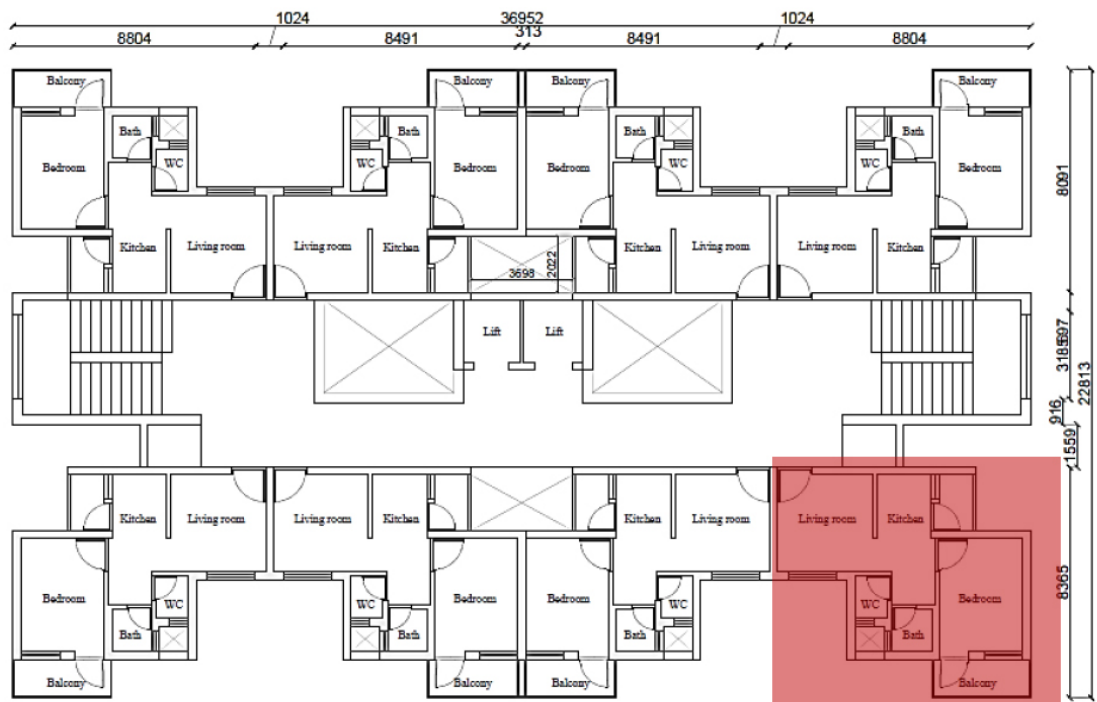
Figure 116: Typical floor plate of a block with longer axis facing north and south directions
