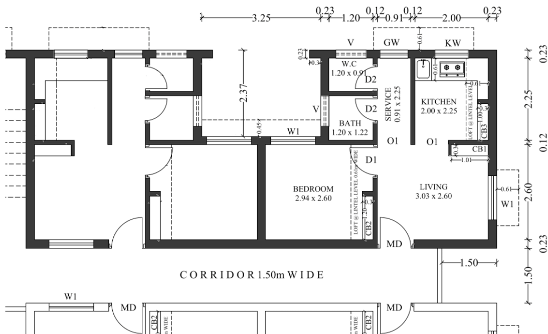
Figure 192: Typical Unit Layout
