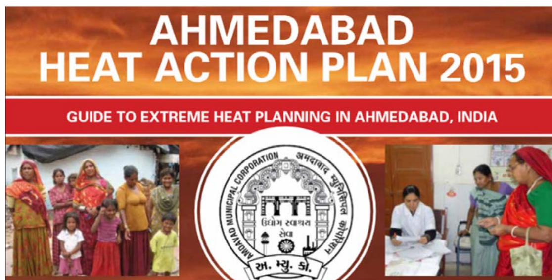
Figure 18: Heat Action Plan launched by the Ahmedabad Municipal Corporation (AMC) and its partners.
