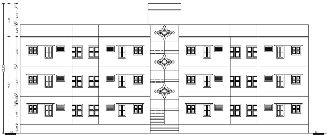
Figure 193: Elevation for Block A1
