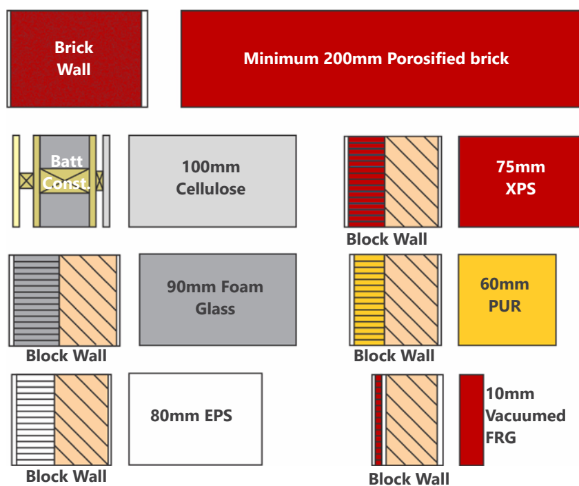
Figure 78: Minimum thickness needed to achieve U value < 0.4 \text{ W/m}^2\text{K} .
