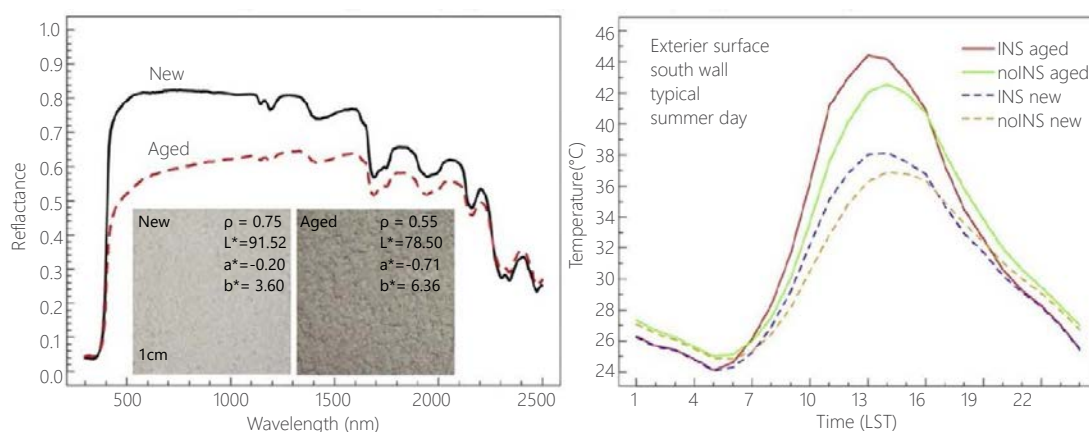
Figure 101: Ageing of high SRI coatings; Source: (Paolini, Zani, Poli, & Zinzi, 2017)
