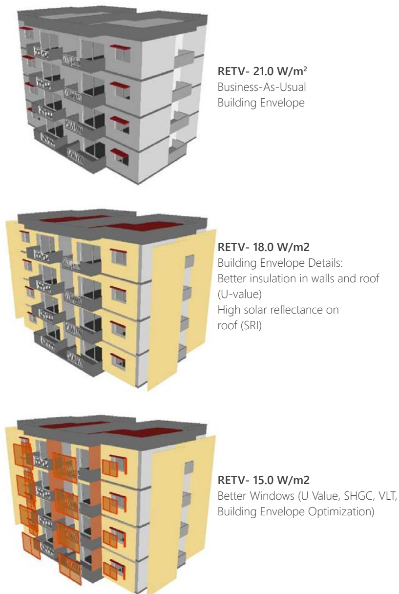
Figure 58: Top- RETV value of typical affordable multifamily residential building; Middle- RETV value after initial envelope optimization strategies; Bottom- RETV value meeting ENS compliance after glazing related optimization strategies
