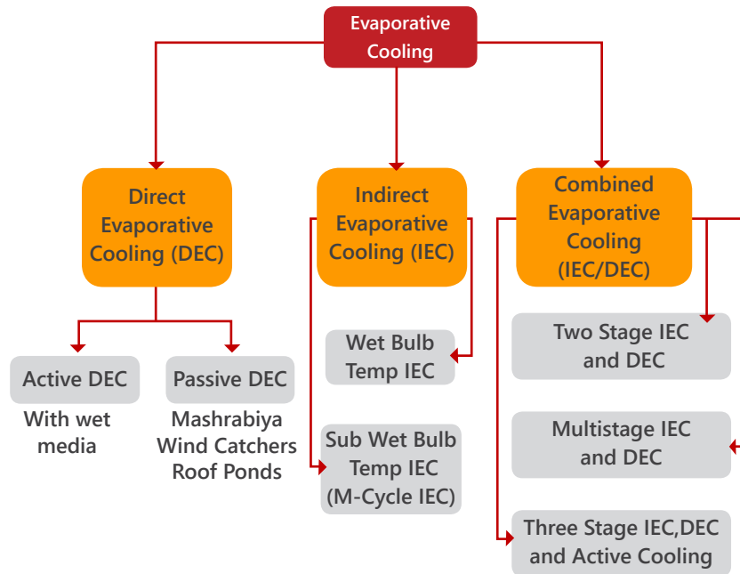
Figure 171: Evaporative cooling
