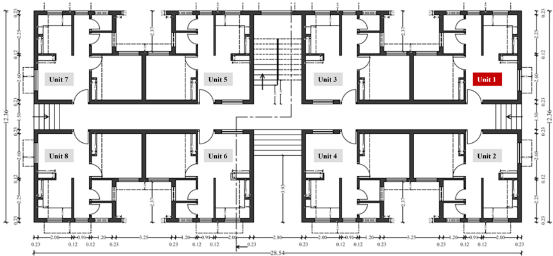
Figure 191: Typical floor plan consisting of 8 units
