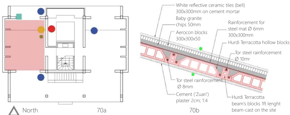
Figure 70: Blessing house architectural and monitoring details; 70a- Position of HOB0 loggers for monitoring the occupied zone; Yellow dot- HOB0 Logger A(RH/Tair/lux), Red dot- HOB0 Logger B 2ch(RH/ Tair), Blue dot- HOB0 Logger D(RH, T), Green dot- Surface temperature sensor; Green square- logger to record open/close state of balcony window; 70b- Roof construction detail;
