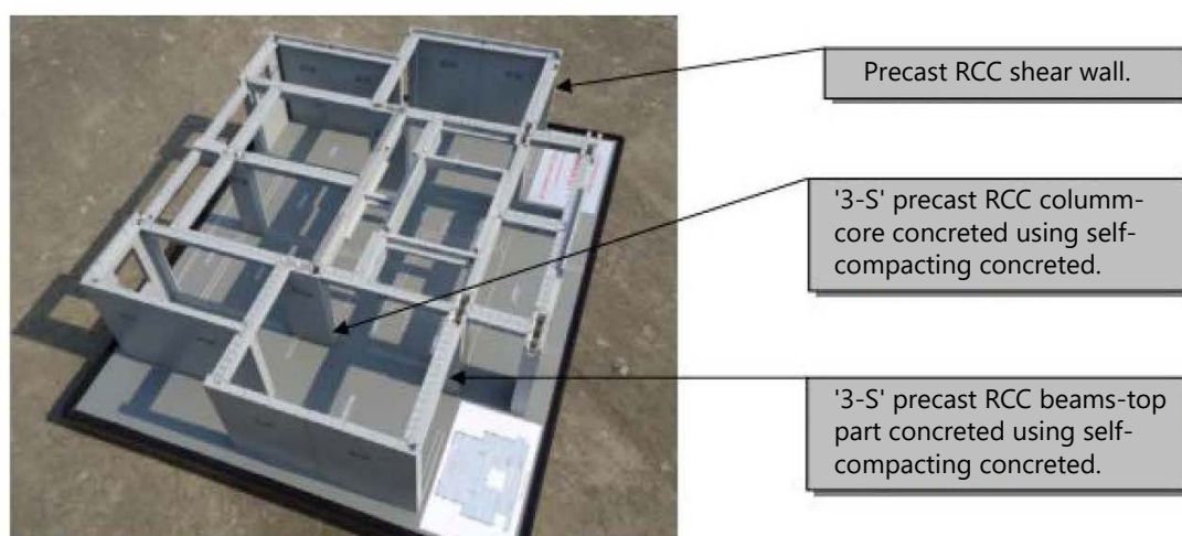
Figure 103: Construction details of LHP Chennai.
