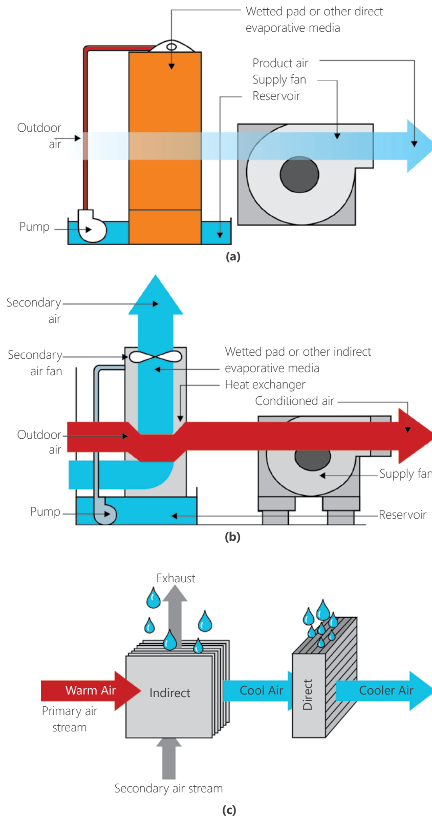
Figure 172: (a) Schematic showing typical Direct Evaporative Cooling System; (b) Schematic showing typical Indirect Evaporative Cooling System; (c) Schematic showing typical two-stage Indirect/Direct Evaporative Cooling System
