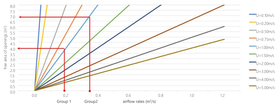
Figure 67: Design Chart DC-03 for single-sided single openings and wind-driven flow. Source: (Cook, et al., 2020)
