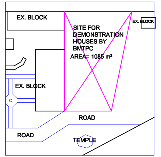
PART SITE PLAN
