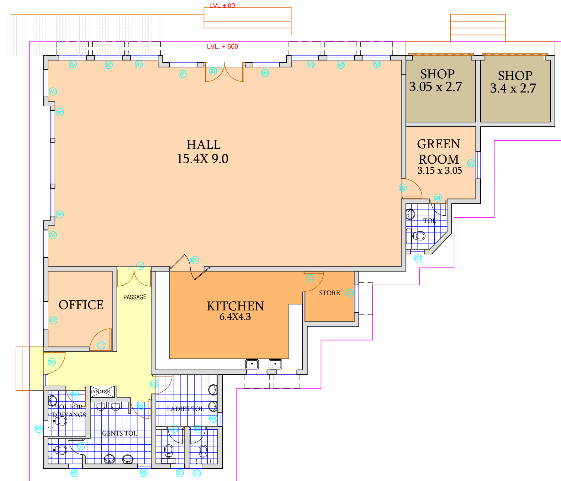
FLOOR PLAN
