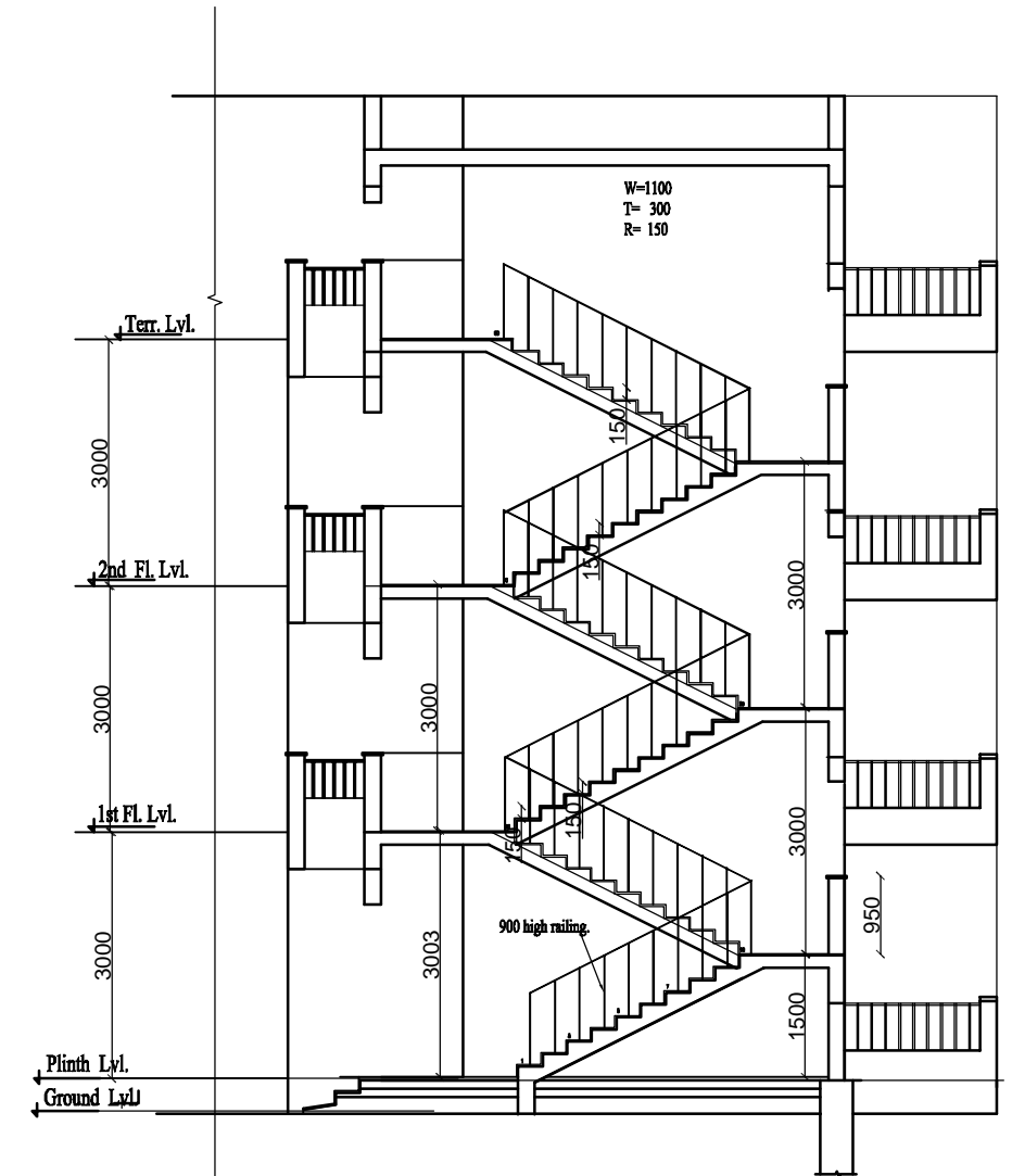
SECTION T-T
