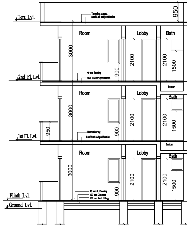
SECTION Y-Y
