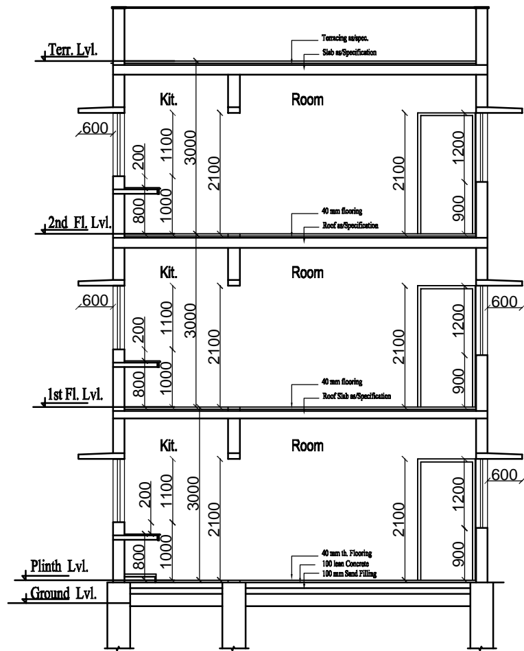
SECTION X-X
