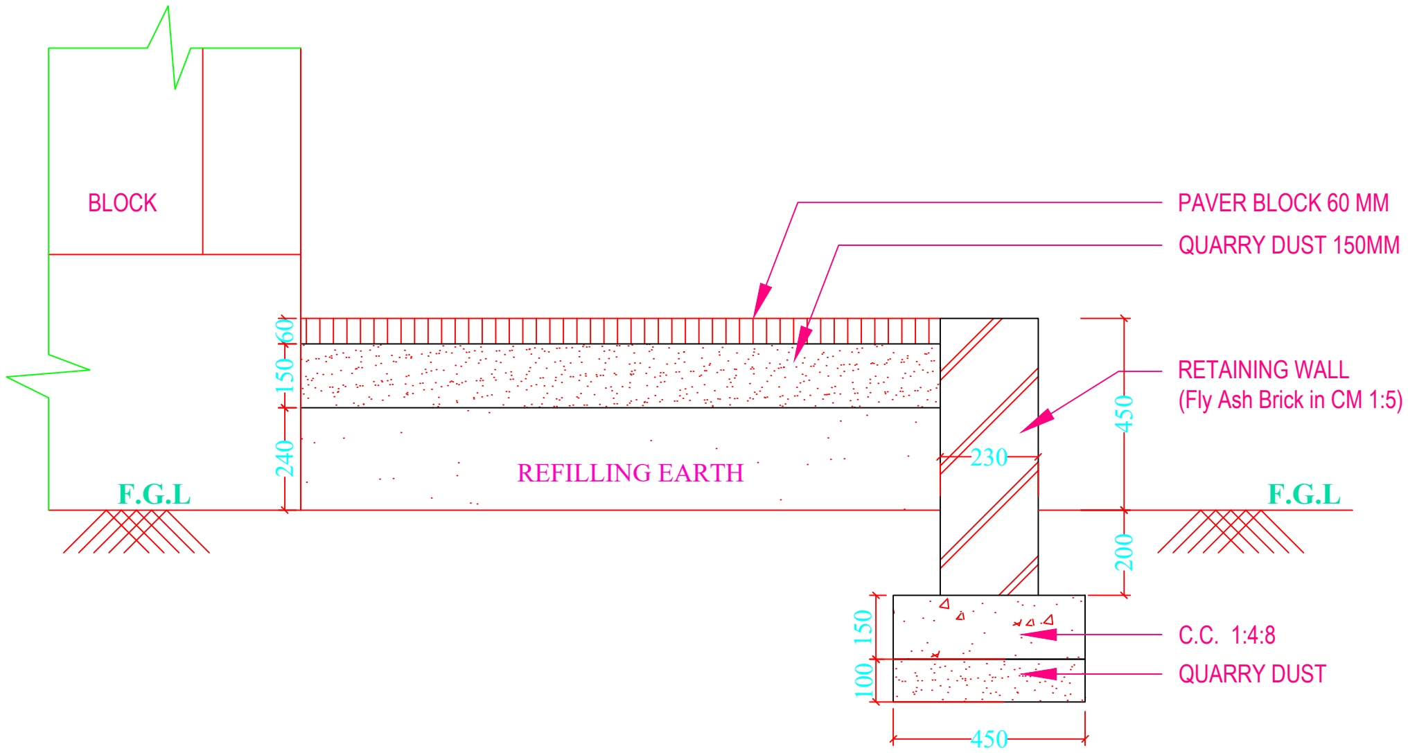
C.S. OF PAVER BLOCK
