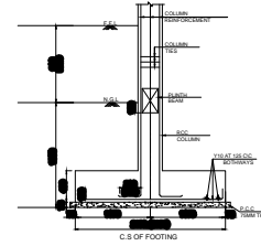
FOOTING DETAIL
