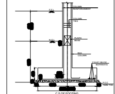
FOOTING DETAIL
